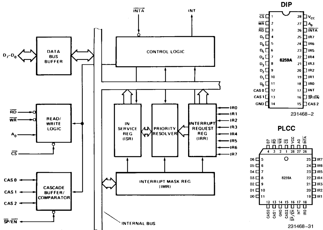
Figure 2. Pin Configurations
